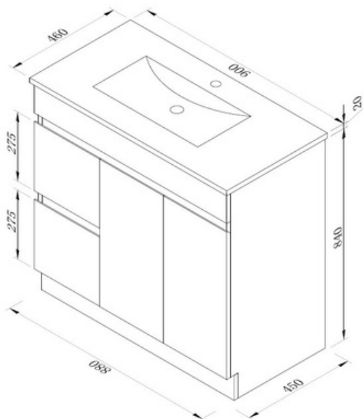
1621731 900mm LEFT HAND DRAWER APPROX : 915W X 460D X 865H
