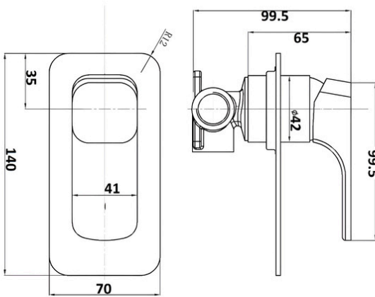
SHOWER / BATH MIXER
