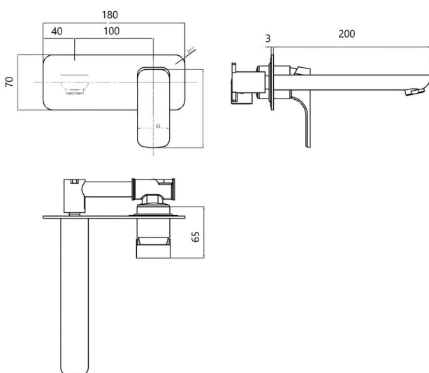
BASIN / BATH MIXER & SPOUT HANDLE ALWAYS ON RHS
