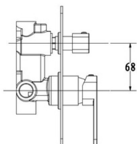
1644684 1644690 DIVERTER SHOWER / BATH MIXER
