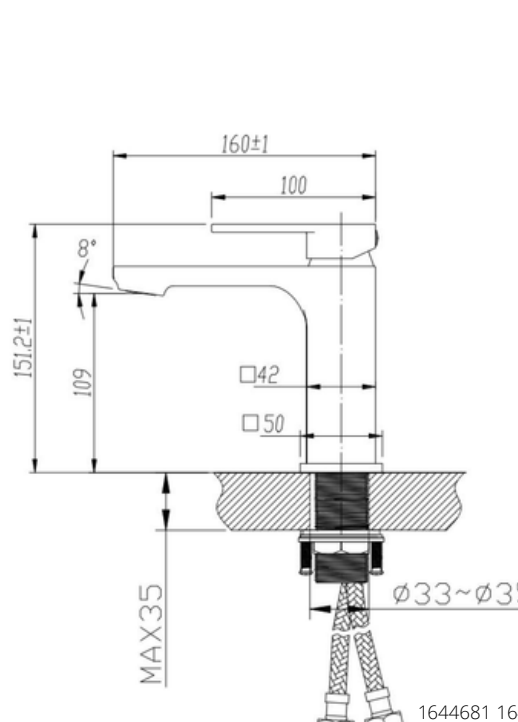
1644681 1644687 BASIN MIXER
