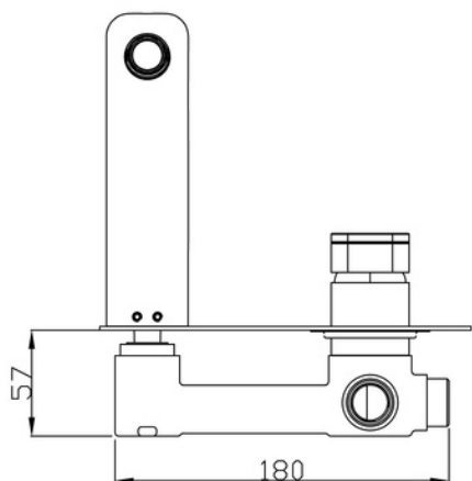
1644681 1644687 BASIN MIXER
